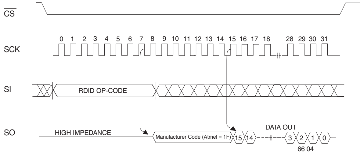
Figure 5-13. RDID Timing
